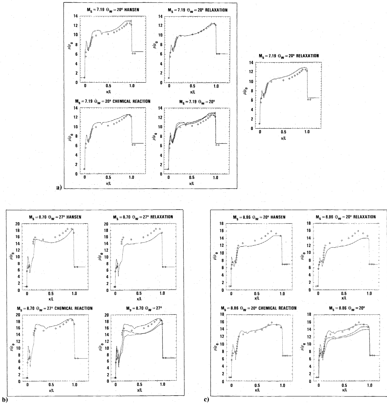
Fig. 6 Plots of density vs distance along the wedge surfaces for the three cases. See Figs. 1 and 2 for definitions of \rho_0 , L . The extra plot for case I corresponds to the calculation with a forced match in state 1'. Diamonds represent experimental data.
