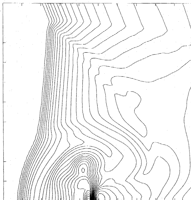
Fig. 7 Continued; blowup plots of the Mach stem region for case III.
