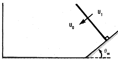
Fig. 1 Schematic diagram for flowfield initialization.
