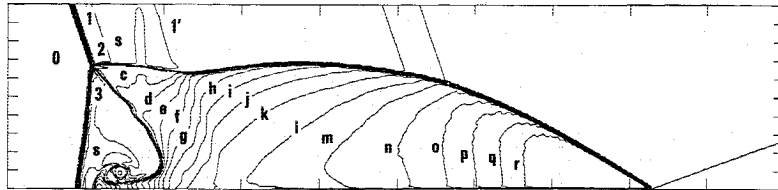
NONEQUILIBRIUM WITHOUT REACTION
