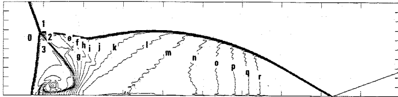
EQUILIBRIUM EOS (HANSEN)
