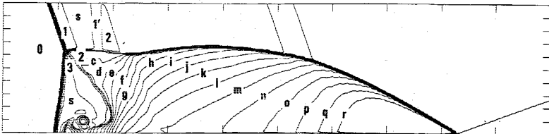
NONEQUILIBRIUM REACTIVE FLOW
