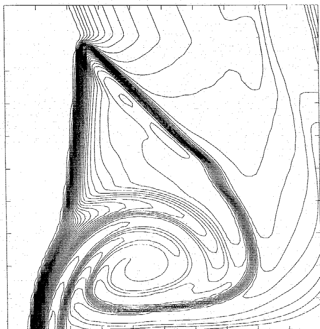
MASS FRACTION OF O
