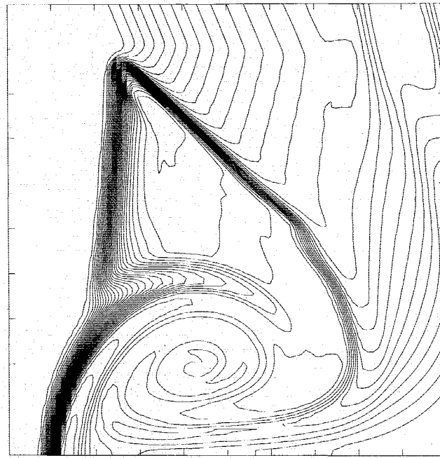
MASS FRACTION OF N 2
