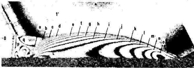
EQUILIBRIUM EOS (HANSEN)
